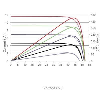
Current-Voltage & Power-Voltage Curves (460W)
